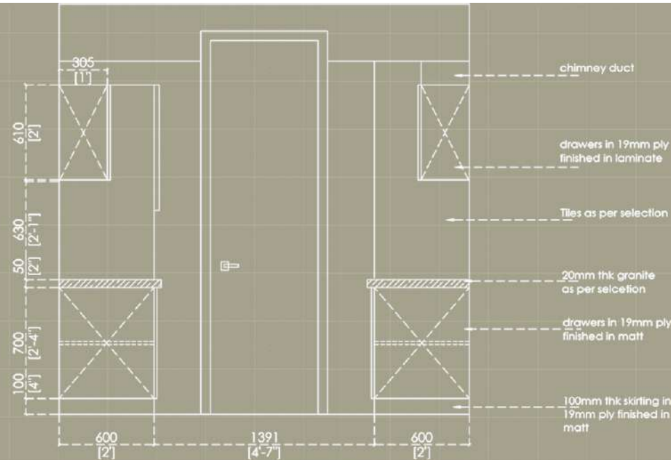
ELEVATION D
