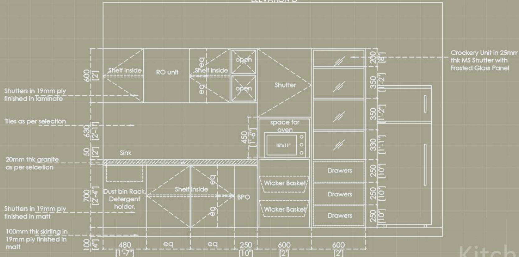
ELEVATION C
